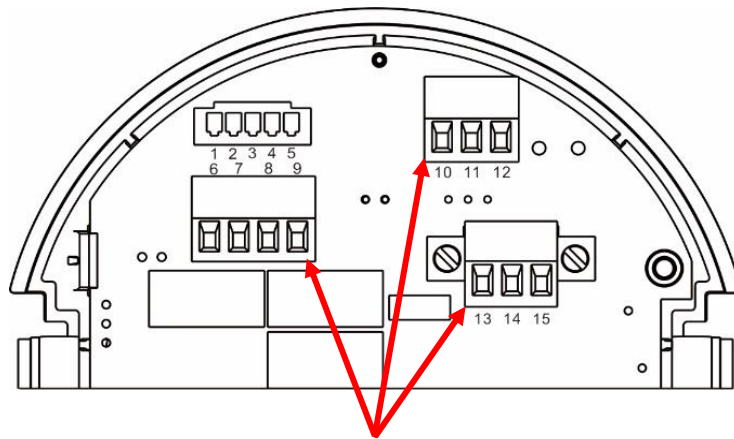
Terminal Blocks
